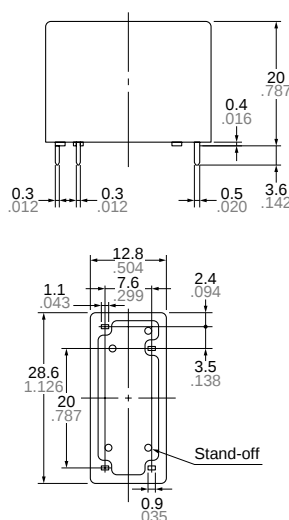
PC board pattern (Copper-side view)
