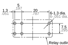
PC board pattern (Copper-side view)
